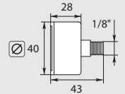
⊙ 40 mm. Housing plastic. Inlet at the back
