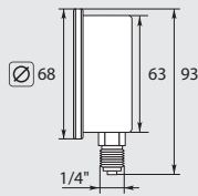
⊙ 63 mm. Housing stainless steel. Inlet at the bottom
